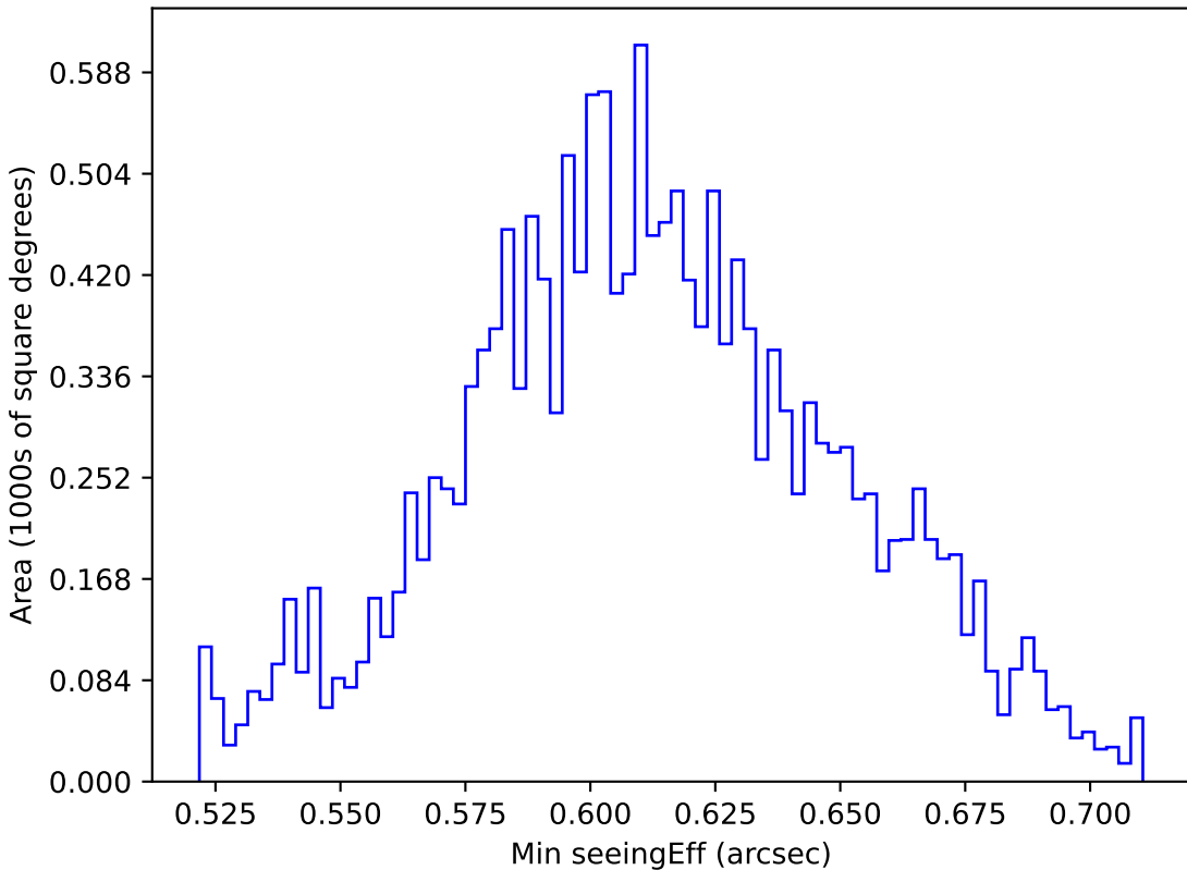
no_magell_roll_v3.4_10yrs WFD z band: Min seeingEff
