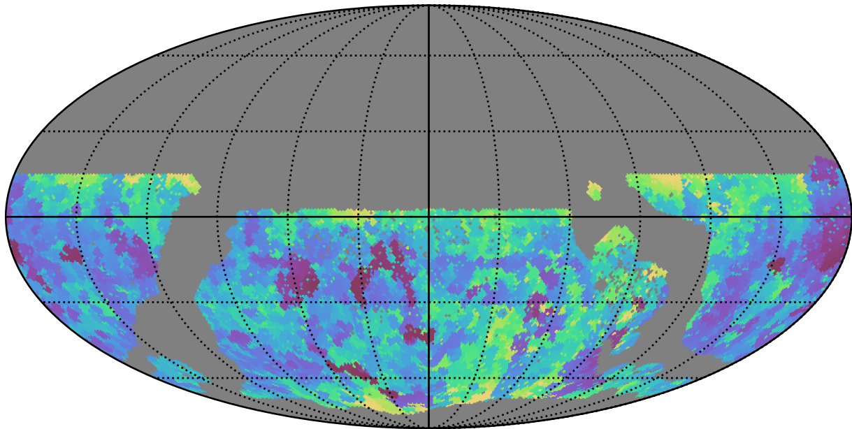
no_magell_roll_v3.4_10yrs WFD u band: Min seeingEff
