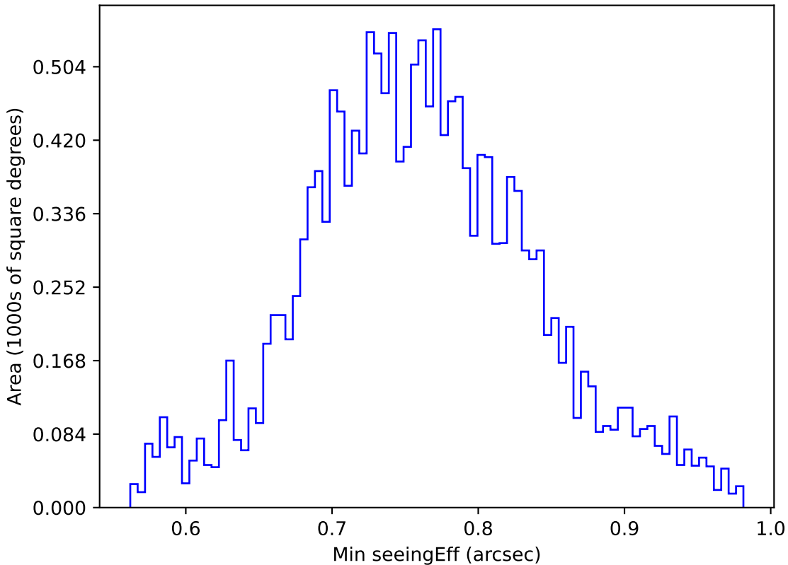
no_magell_roll_v3.4_10yrs WFD u band: Min seeingEff
