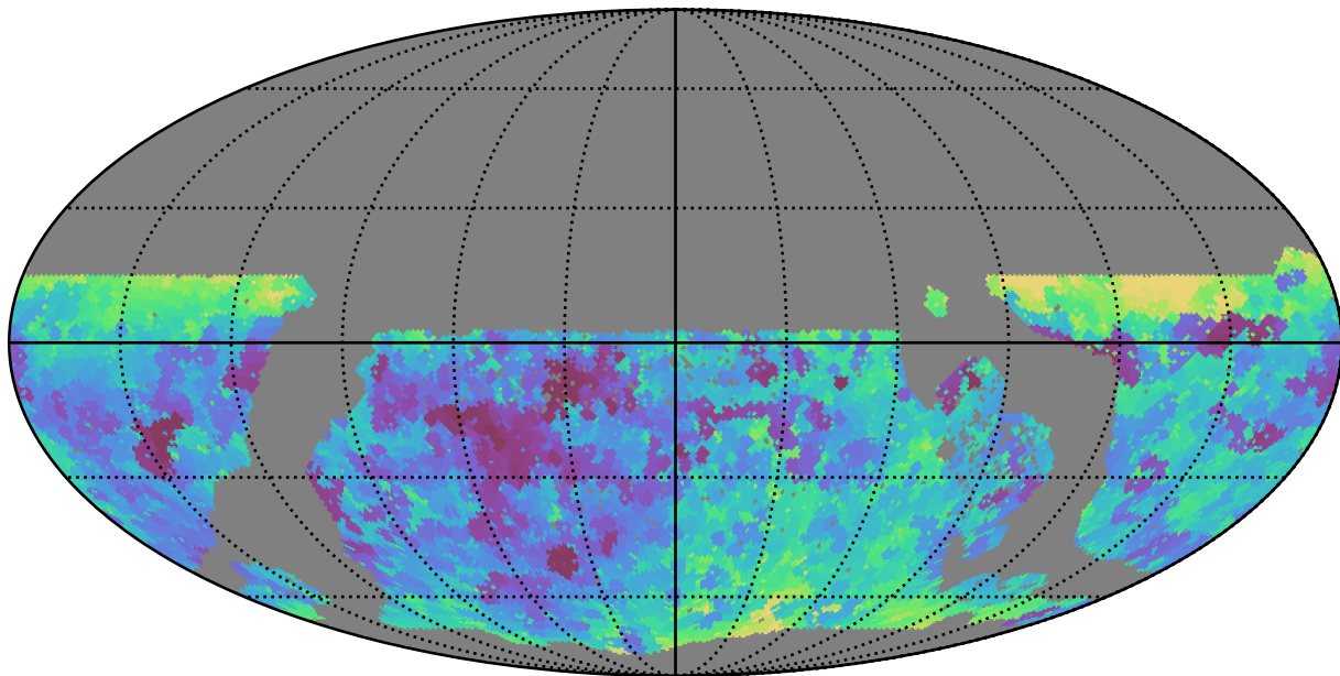
no_magell_roll_v3.4_10yrs WFD r band: Min seeingEff
