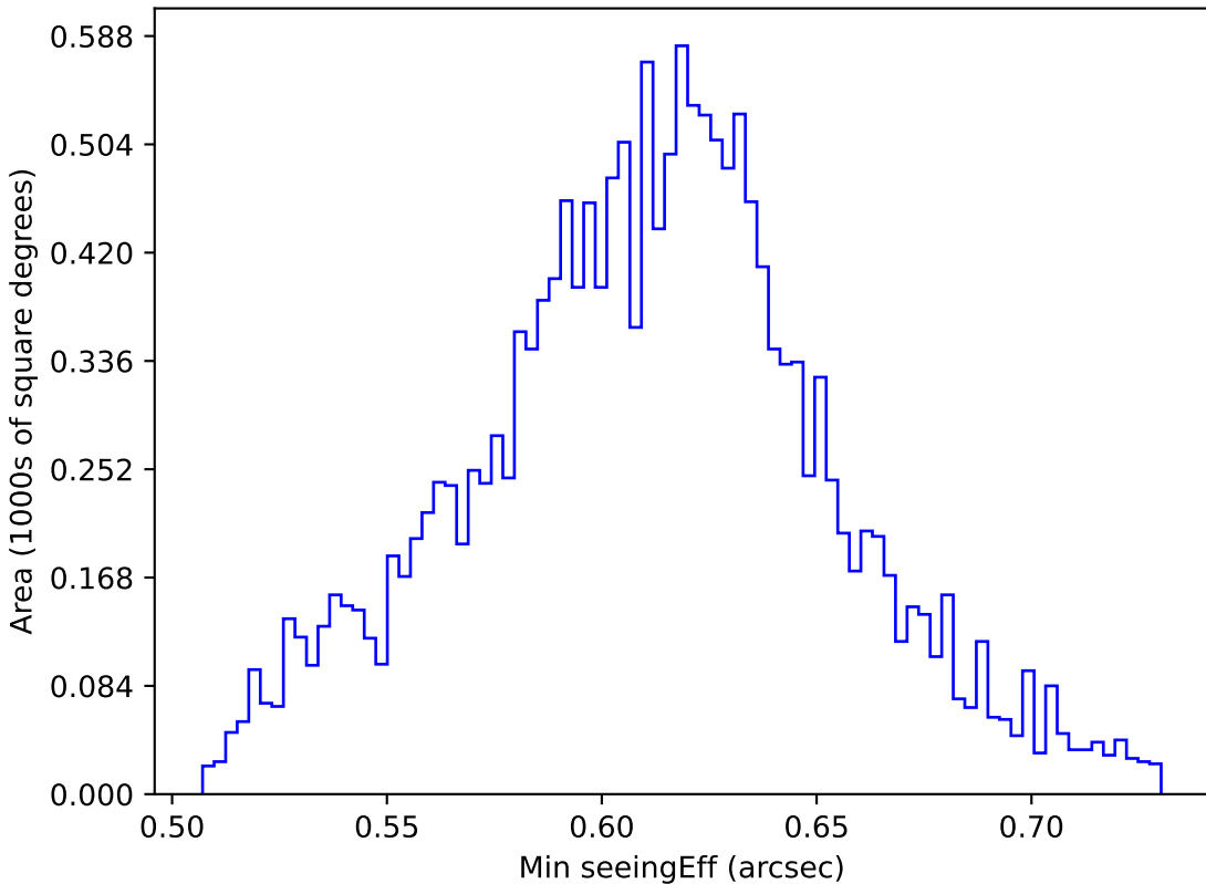
no_magell_roll_v3.4_10yrs WFD r band: Min seeingEff
