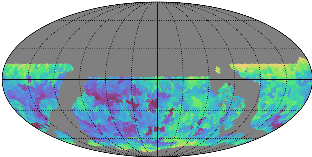
no_magell_roll_v3.4_10yrs WFD i band: Min seeingEff
