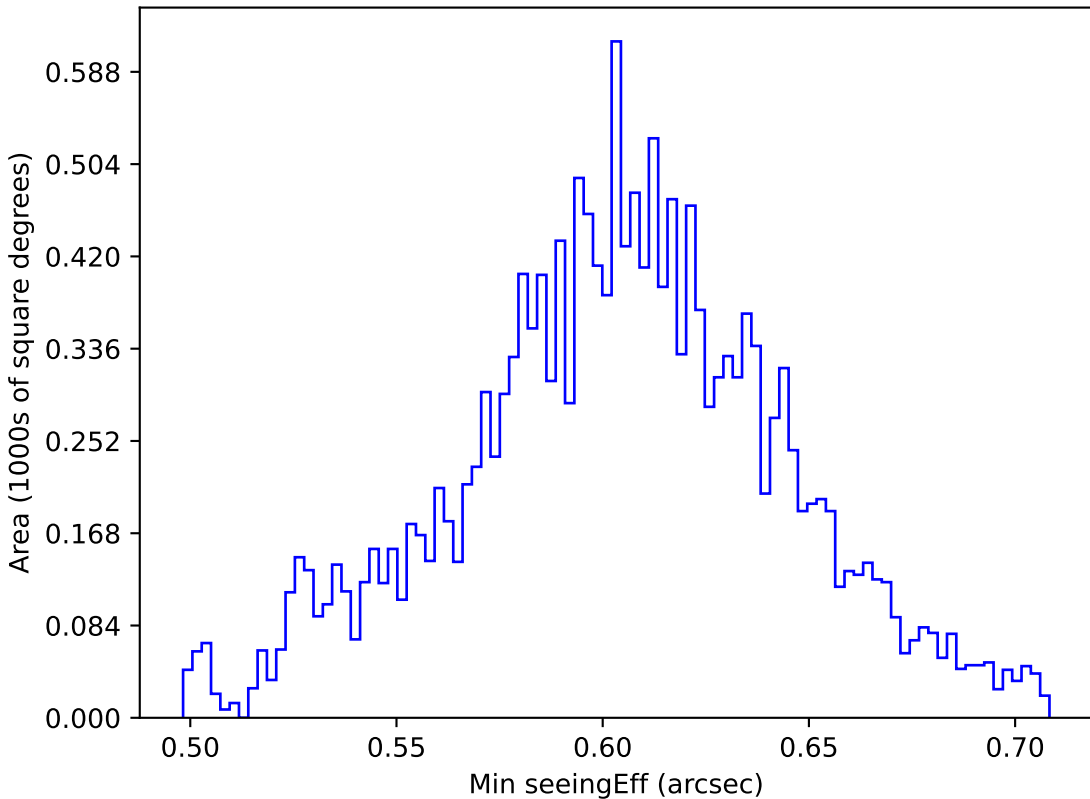
no_magell_roll_v3.4_10yrs WFD i band: Min seeingEff
