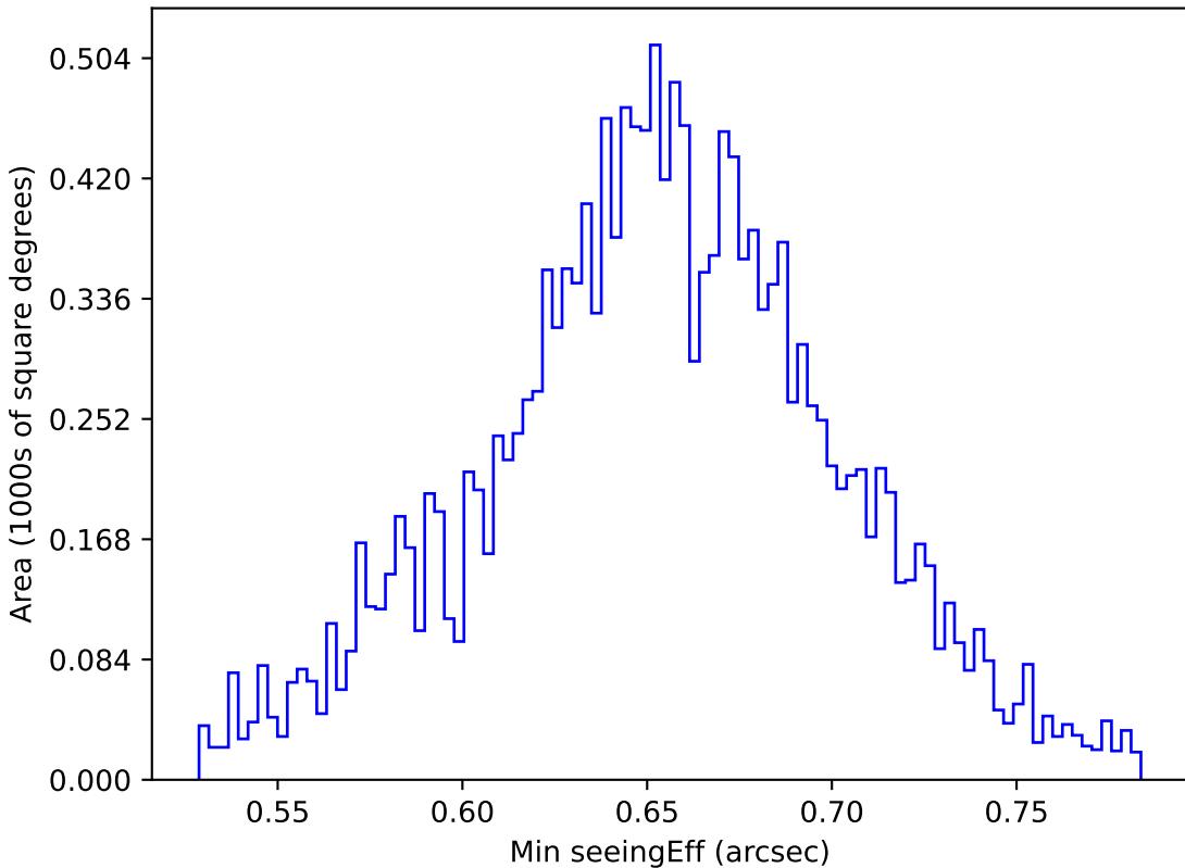
no_magell_roll_v3.4_10yrs WFD g band: Min seeingEff
