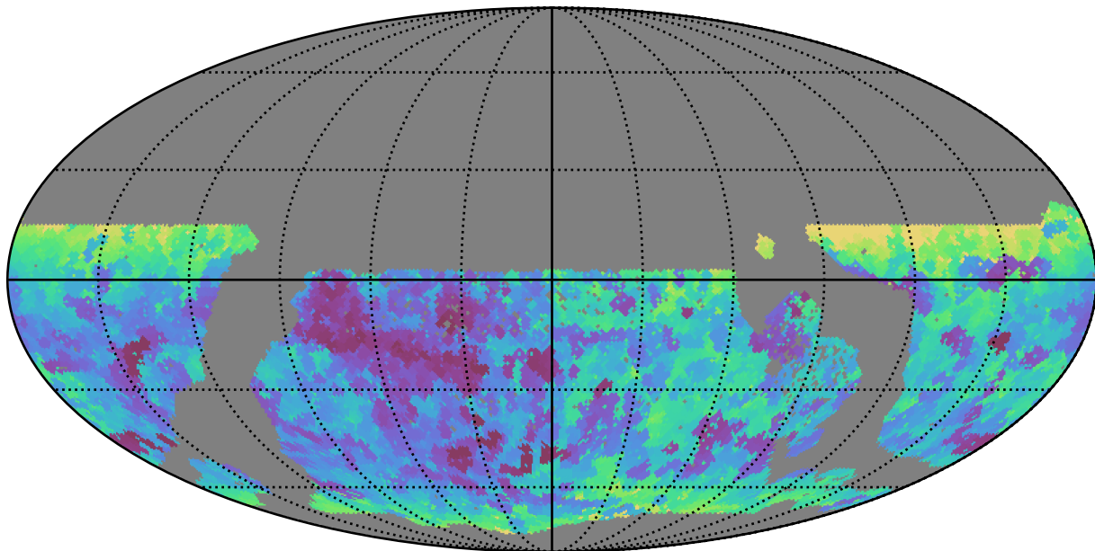
no_magell_roll_v3.4_10yrs WFD all bands: Min seeingEff
