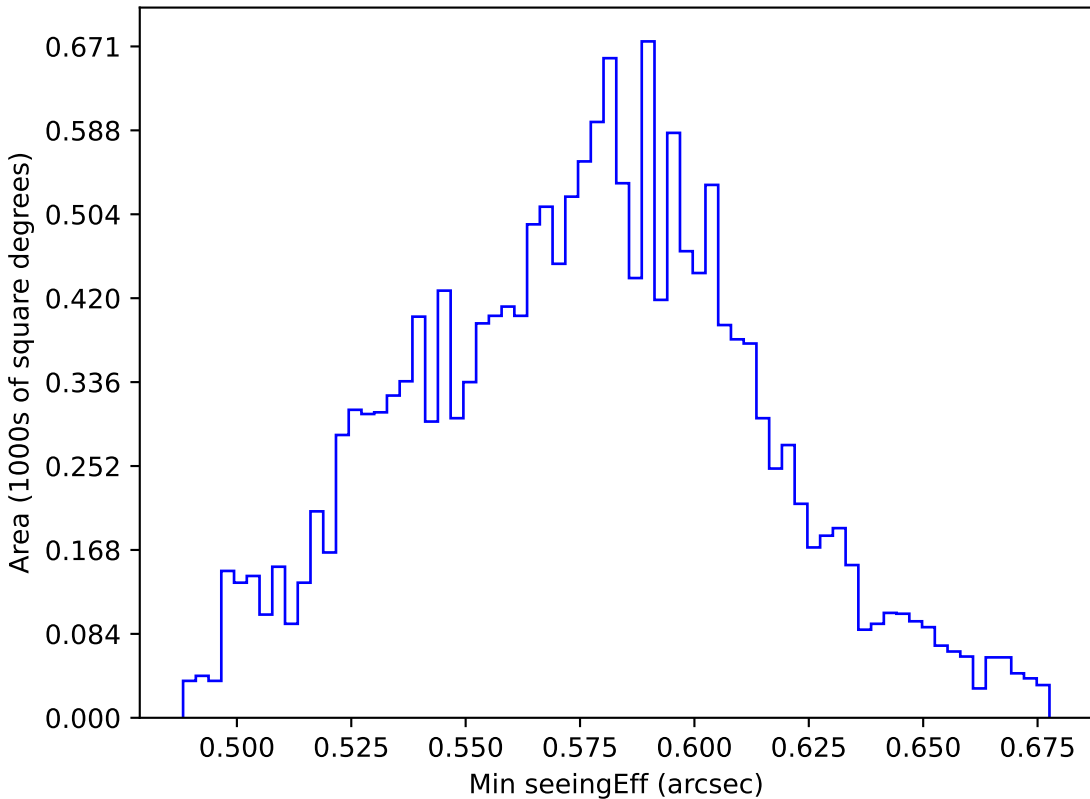
no_magell_roll_v3.4_10yrs WFD all bands: Min seeingEff
