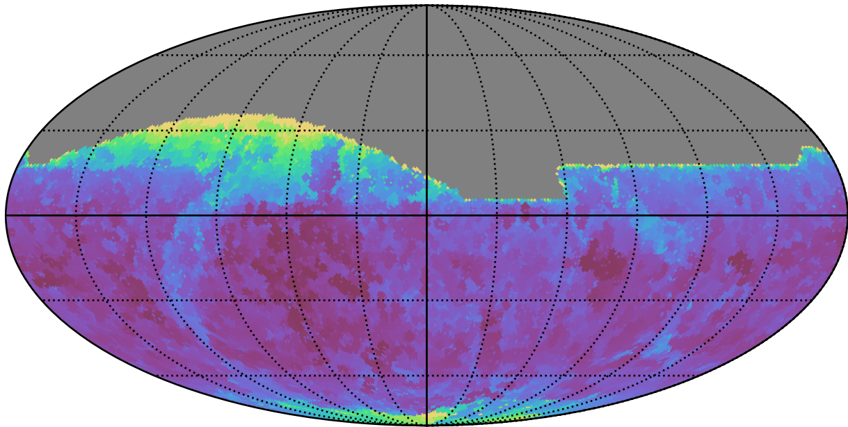
no_magell_roll_v3.4_10yrs All sky z band: Min seeingEff
