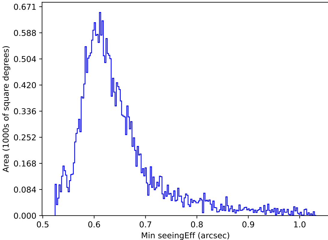
no_magell_roll_v3.4_10yrs All sky z band: Min seeingEff
