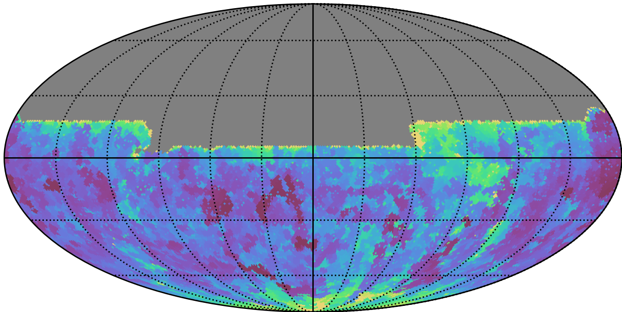
no_magell_roll_v3.4_10yrs All sky u band: Min seeingEff
