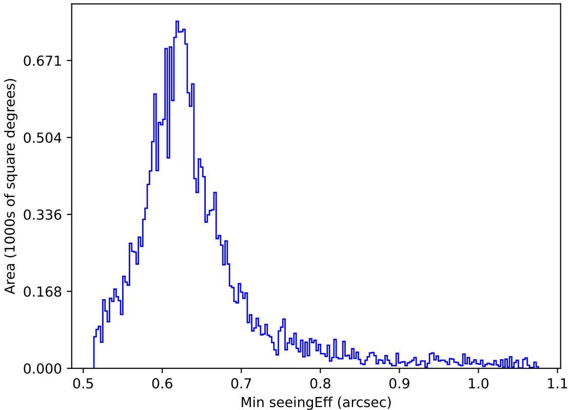
no_magell_roll_v3.4_10yrs All sky r band: Min seeingEff
