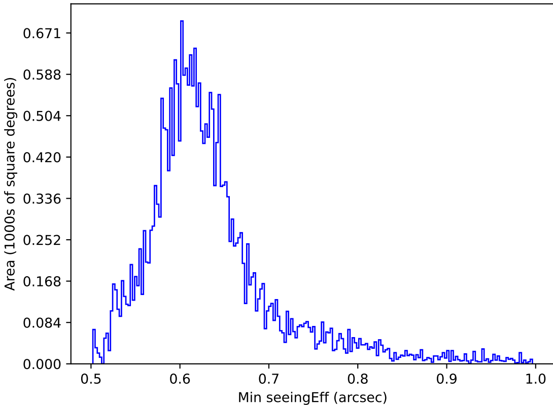
no_magell_roll_v3.4_10yrs All sky i band: Min seeingEff
