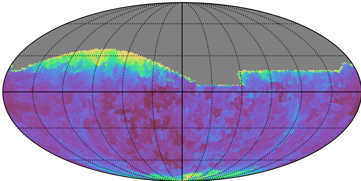
no_magell_roll_v3.4_10yrs All sky g band: Min seeingEff
