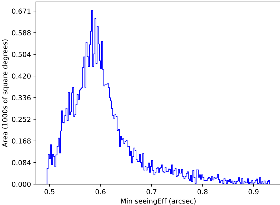
no_magell_roll_v3.4_10yrs All sky all bands: Min seeingEff
