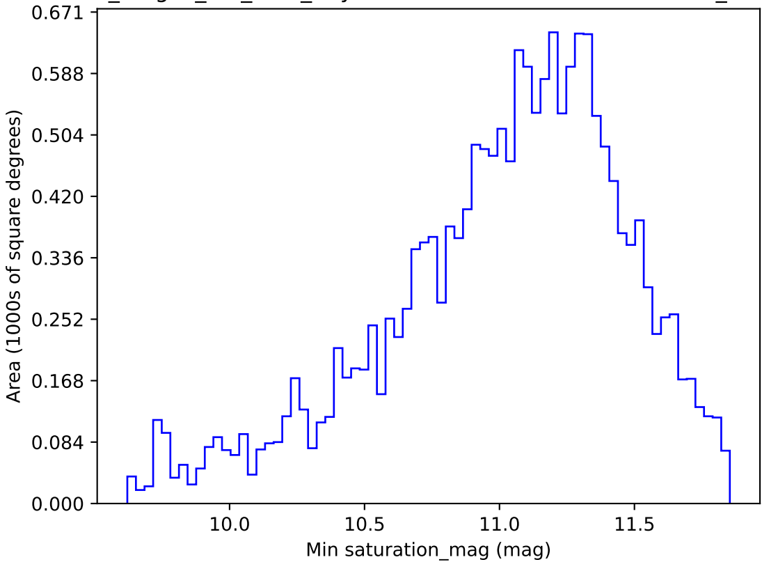
no_magell_roll_v3.4_10yrs WFD all bands: Min saturation_mag
