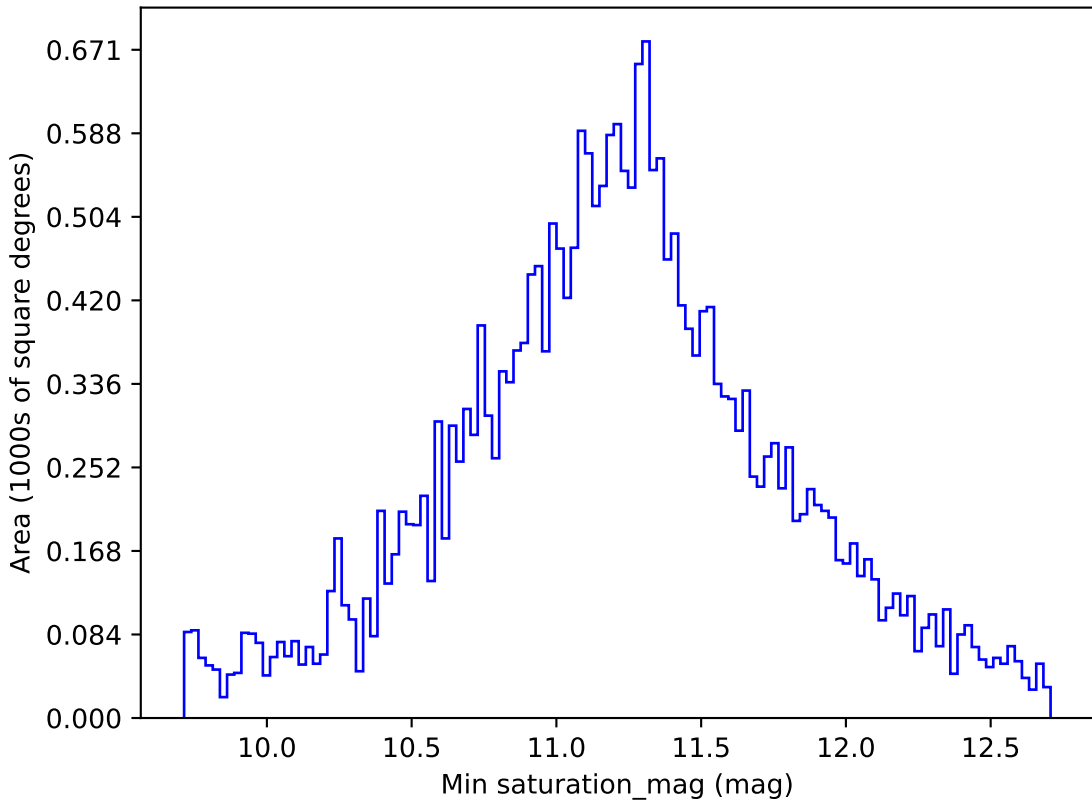
no_magell_roll_v3.4_10yrs All sky all bands: Min saturation_mag
