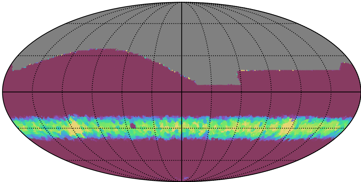
no_magell_roll_v3.4_10yrs All sky all bands: Min normairmass
