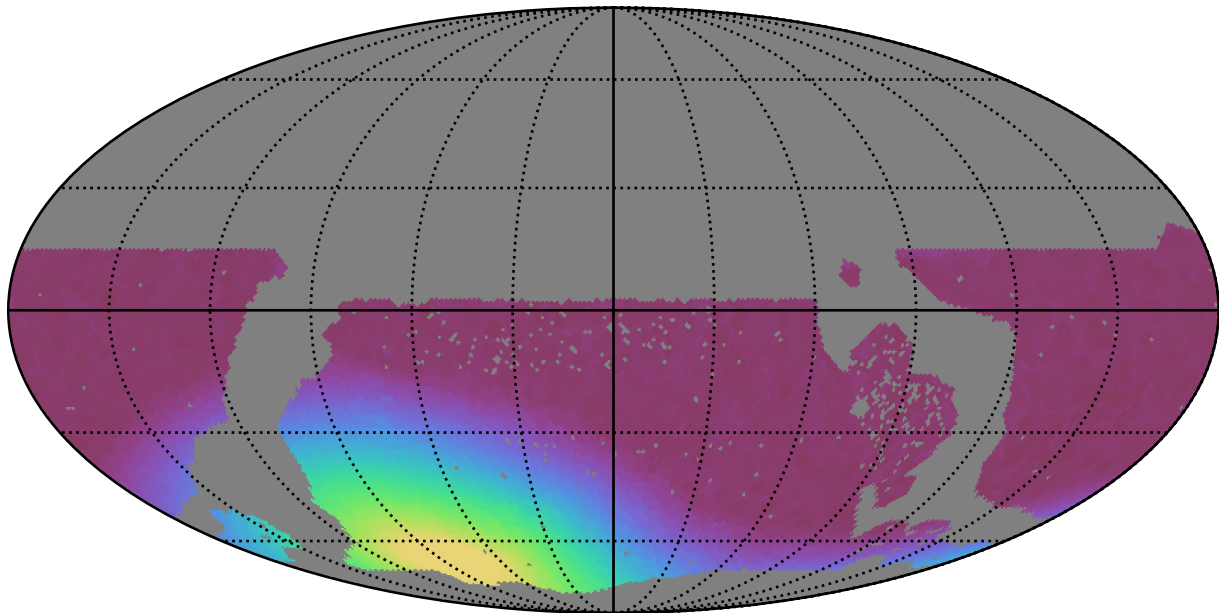
no_magell_roll_v3.4_10yrs WFD all bands: Min moonDistance
