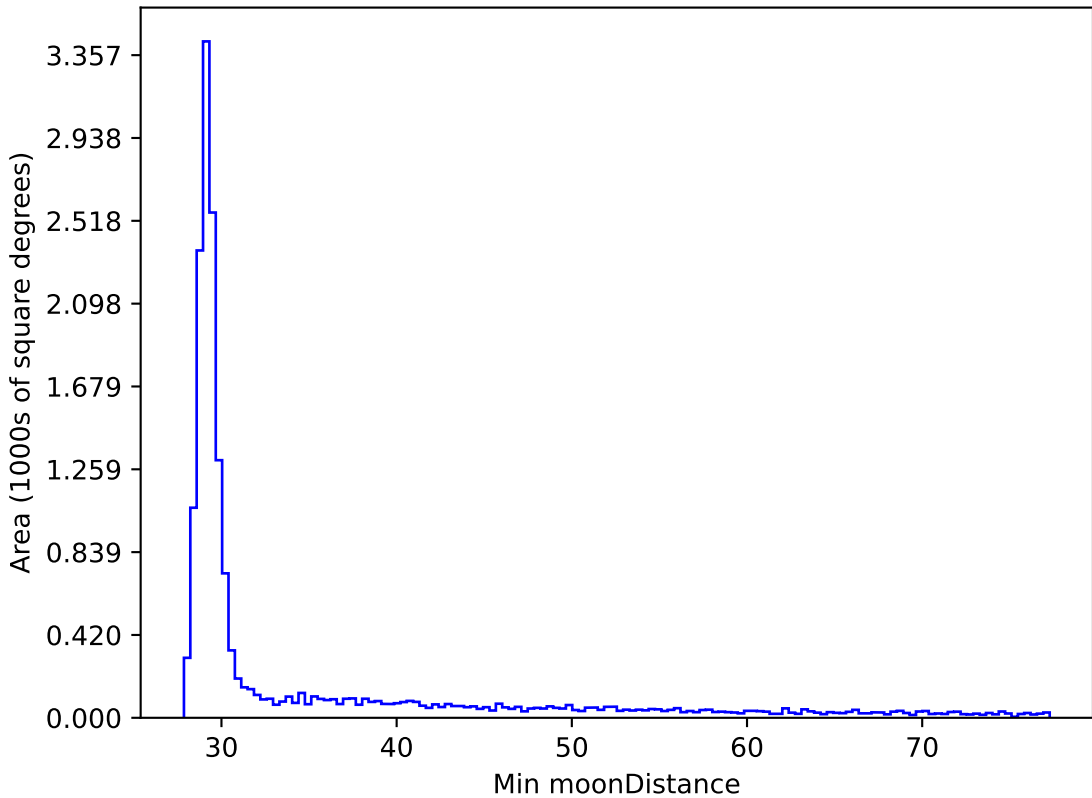
no_magell_roll_v3.4_10yrs WFD all bands: Min moonDistance
