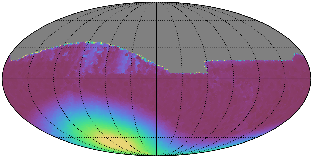
no_magell_roll_v3.4_10yrs All sky all bands: Min moonDistance
