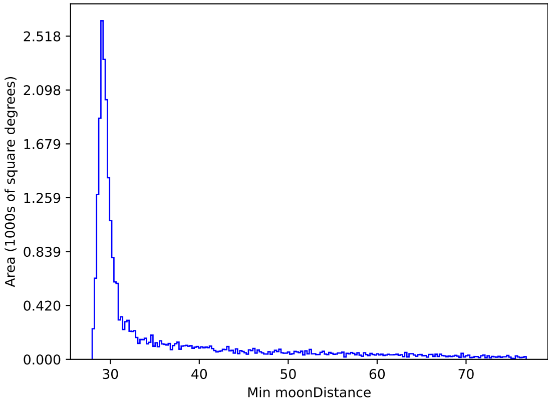
no_magell_roll_v3.4_10yrs All sky all bands: Min moonDistance
