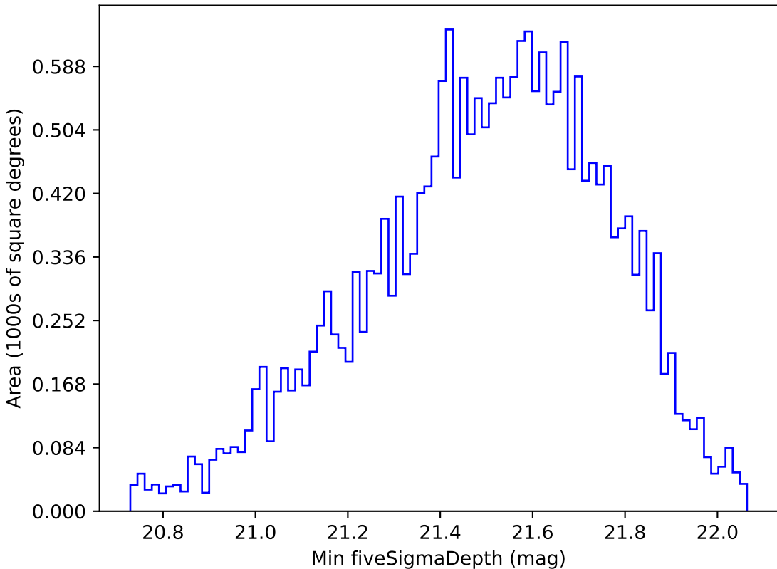
no_magell_roll_v3.4_10yrs Yr 1 y band: Min fiveSigmaDepth
