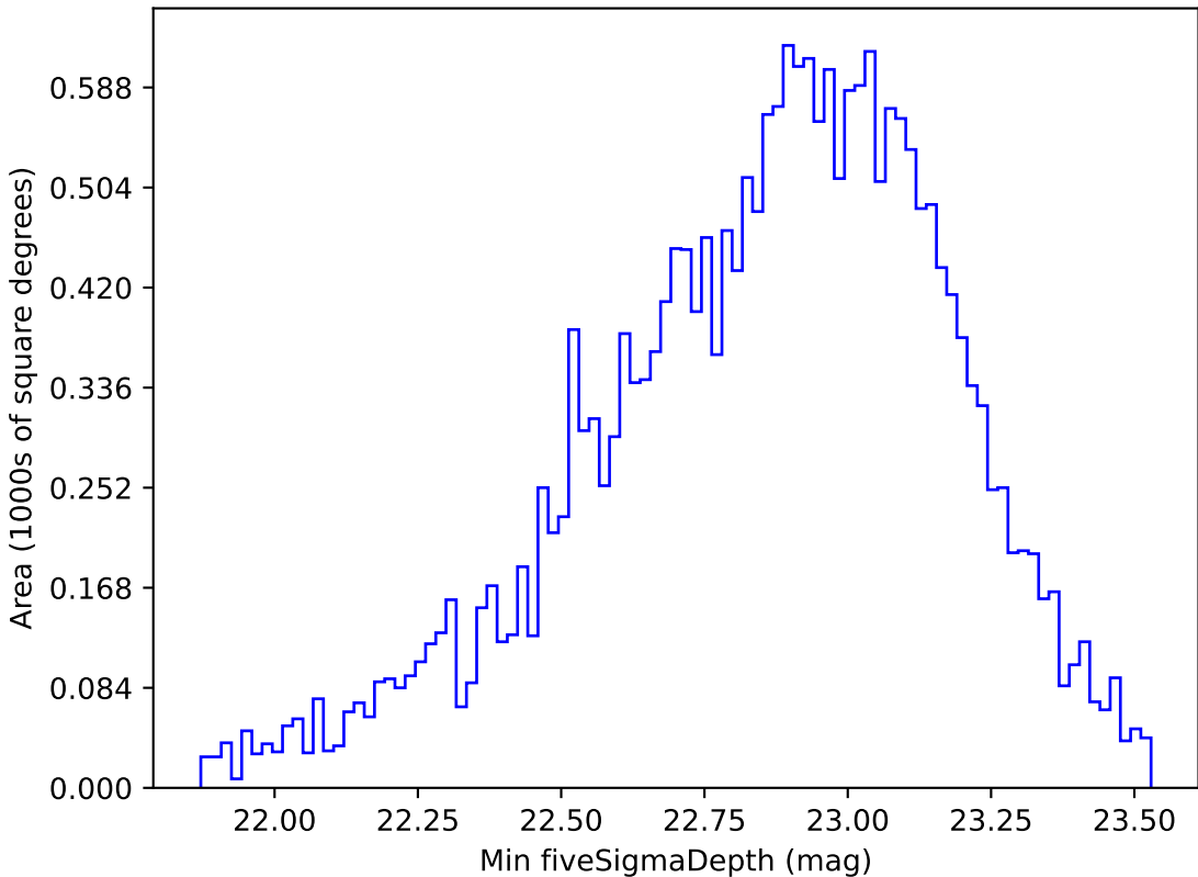
no_magell_roll_v3.4_10yrs Yr 1 u band: Min fiveSigmaDepth
