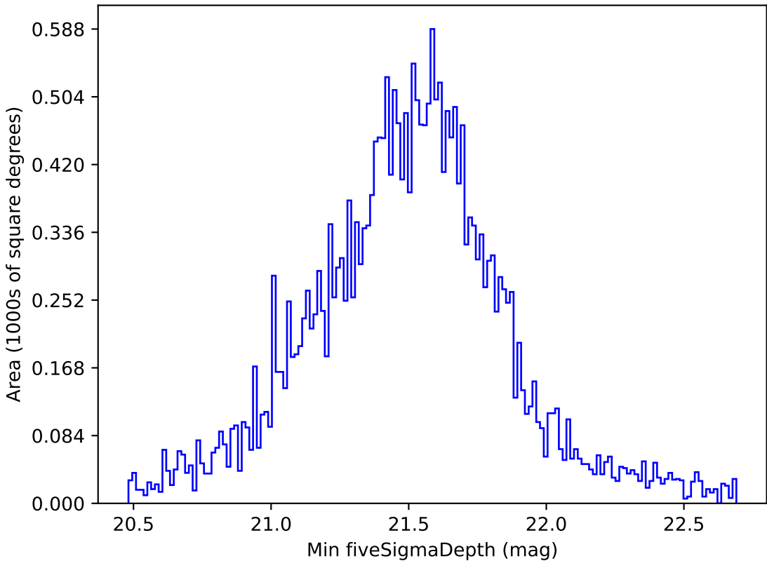
no_magell_roll_v3.4_10yrs Yr 1 all bands: Min fiveSigmaDepth
