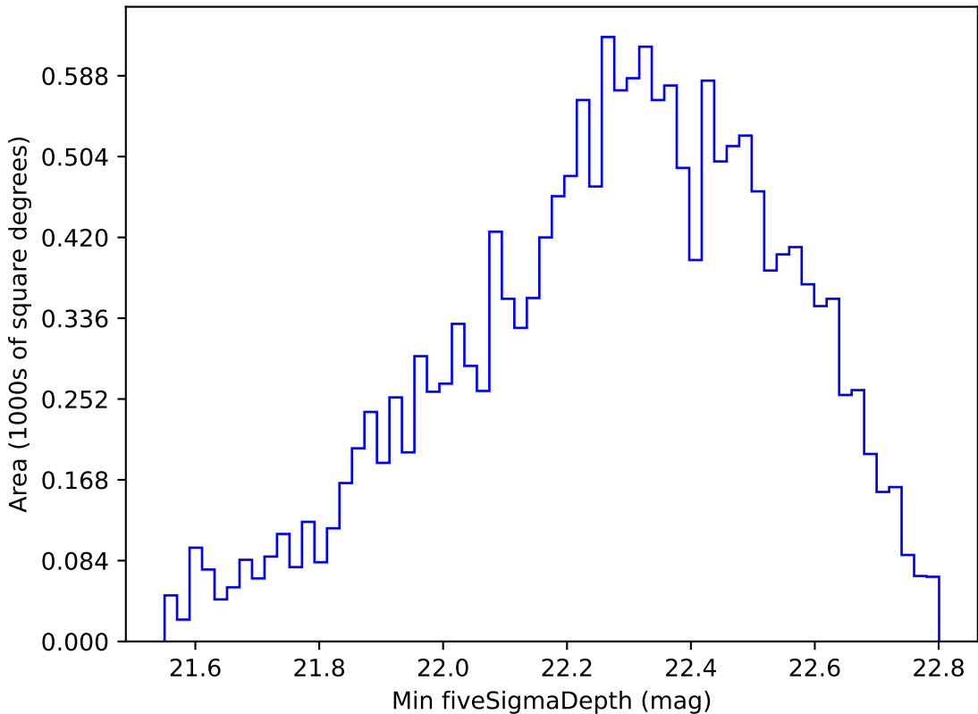
no_magell_roll_v3.4_10yrs WFD u band: Min fiveSigmaDepth
