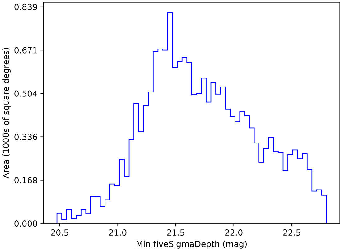
no_magell_roll_v3.4_10yrs WFD i band: Min fiveSigmaDepth
