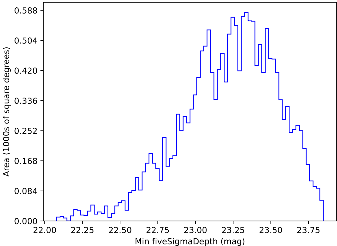
no_magell_roll_v3.4_10yrs WFD g band: Min fiveSigmaDepth
