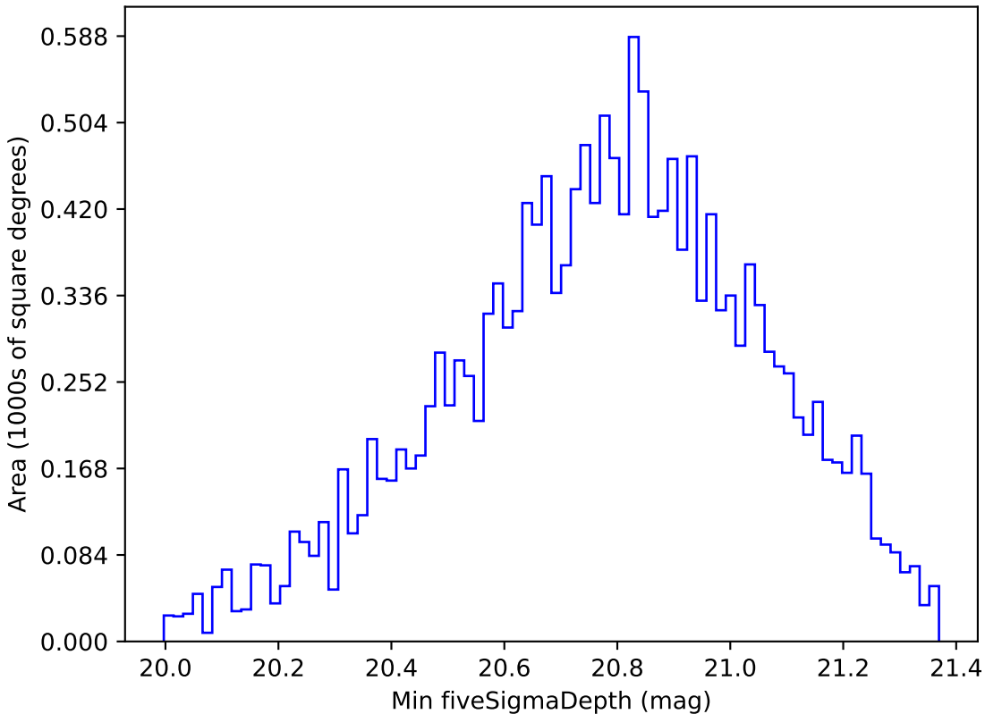
no_magell_roll_v3.4_10yrs WFD all bands: Min fiveSigmaDepth
