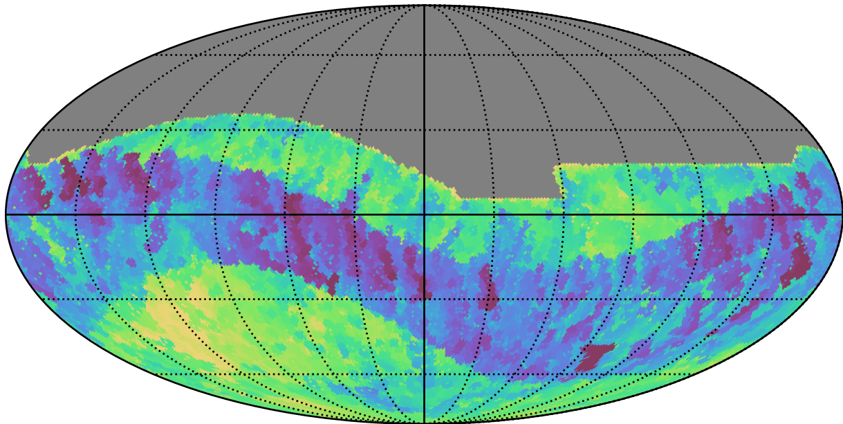
no_magell_roll_v3.4_10yrs All sky z band: Min fiveSigmaDepth
