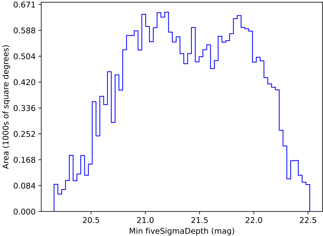
no_magell_roll_v3.4_10yrs All sky z band: Min fiveSigmaDepth
