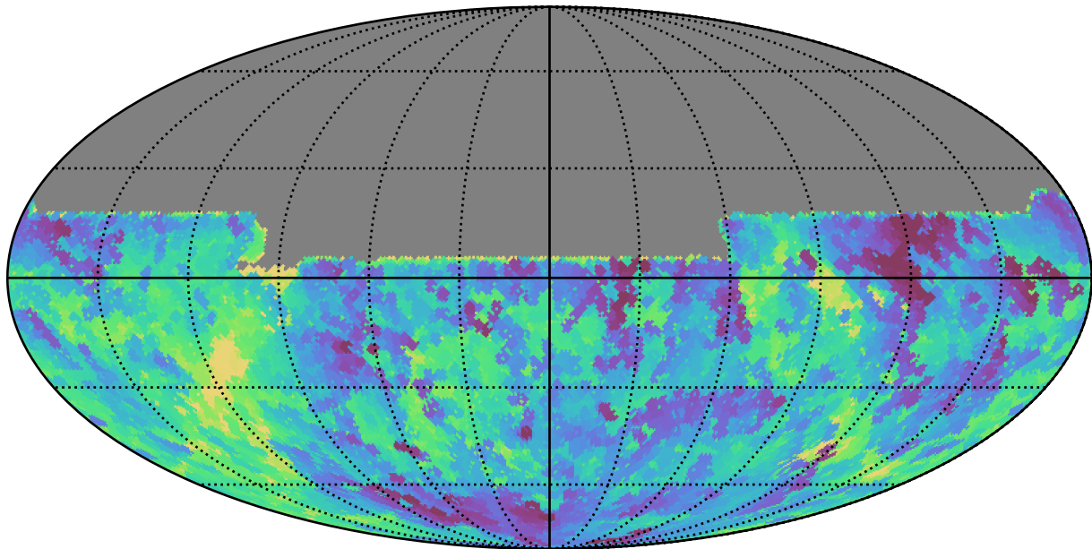
no_magell_roll_v3.4_10yrs All sky u band: Min fiveSigmaDepth
