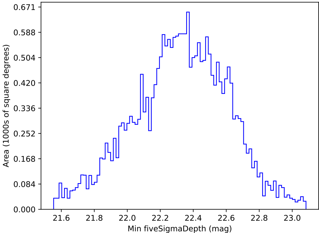
no_magell_roll_v3.4_10yrs All sky u band: Min fiveSigmaDepth
