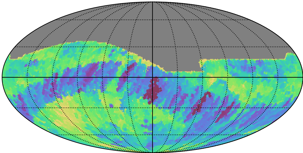
no_magell_roll_v3.4_10yrs All sky r band: Min fiveSigmaDepth
