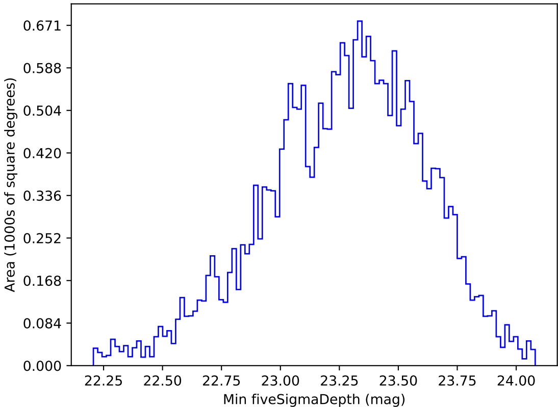
no_magell_roll_v3.4_10yrs All sky g band: Min fiveSigmaDepth
