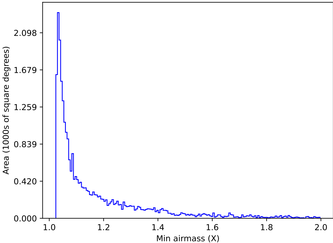
no_magell_roll_v3.4_10yrs Yr 1 z band: Min airmass
