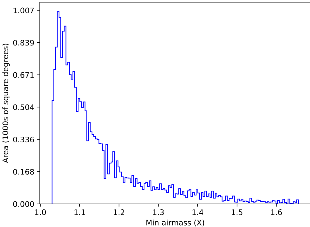
no_magell_roll_v3.4_10yrs Yr 1 u band: Min airmass
