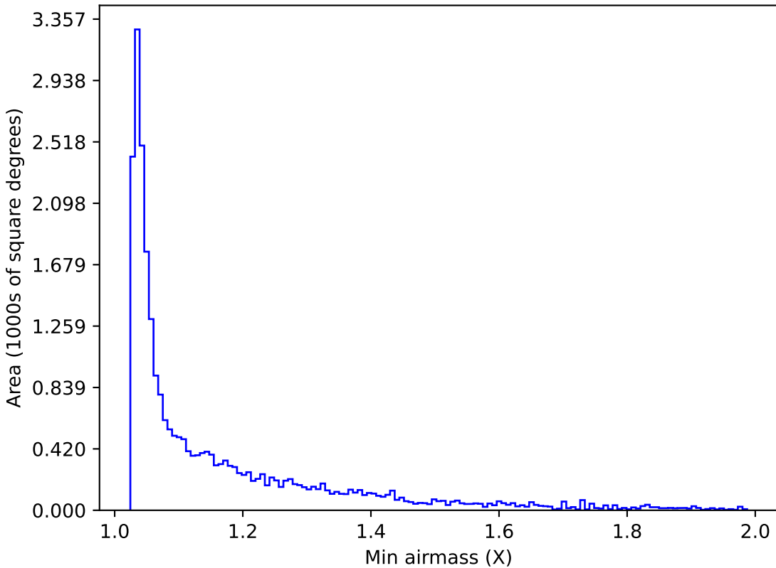
no_magell_roll_v3.4_10yrs Yr 1 i band: Min airmass
