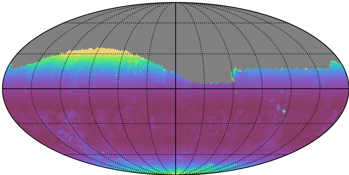
no_magell_roll_v3.4_10yrs Yr 1 g band: Min airmass
