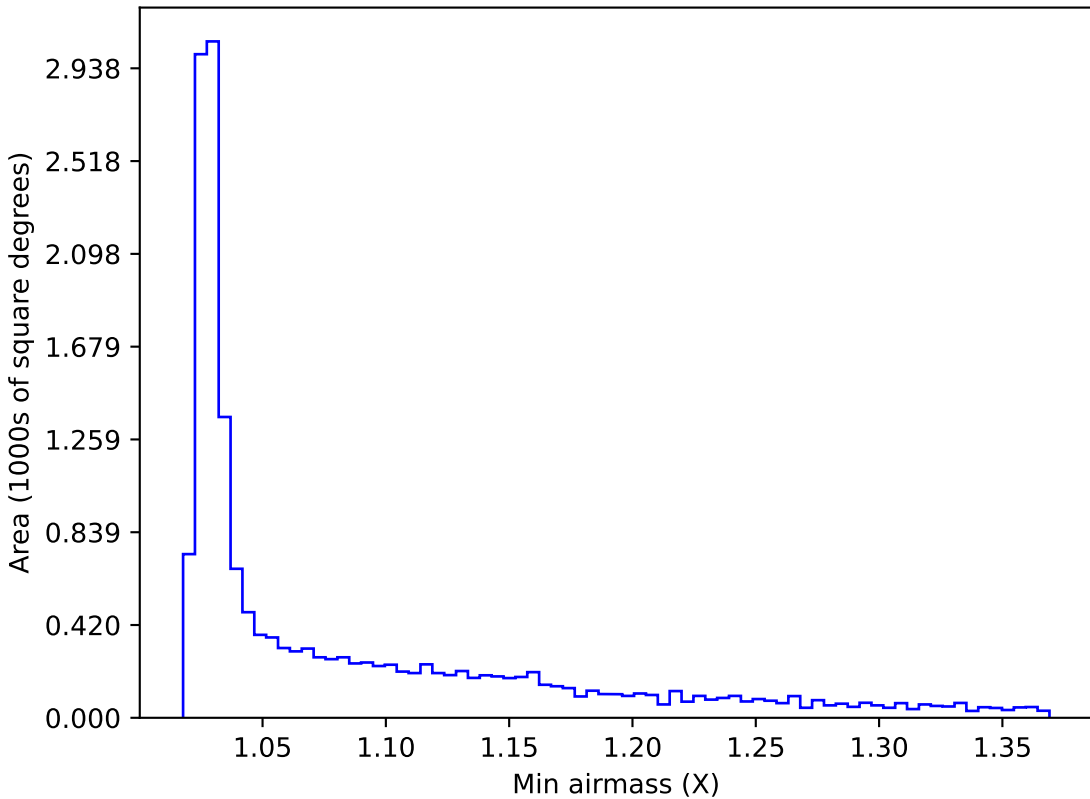
no_magell_roll_v3.4_10yrs WFD z band: Min airmass
