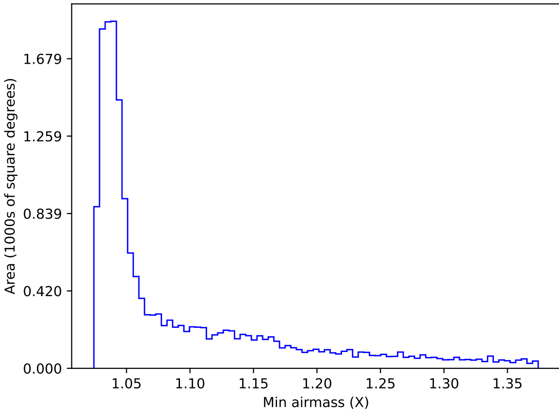
no_magell_roll_v3.4_10yrs WFD u band: Min airmass
