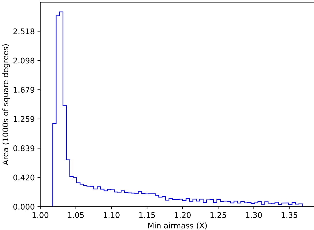
no_magell_roll_v3.4_10yrs WFD r band: Min airmass
