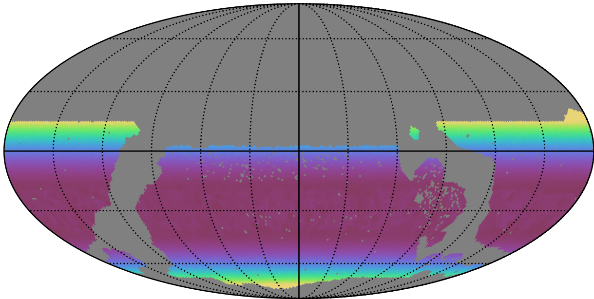
no_magell_roll_v3.4_10yrs WFD i band: Min airmass
