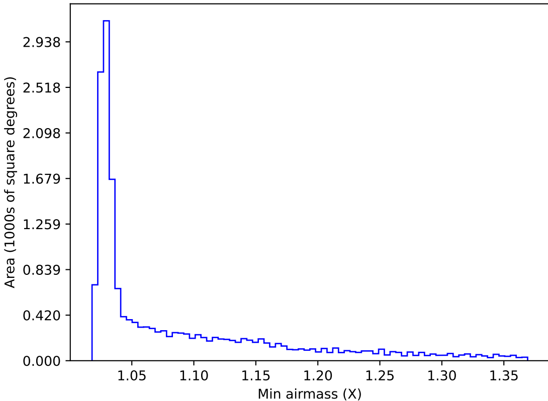
no_magell_roll_v3.4_10yrs WFD i band: Min airmass
