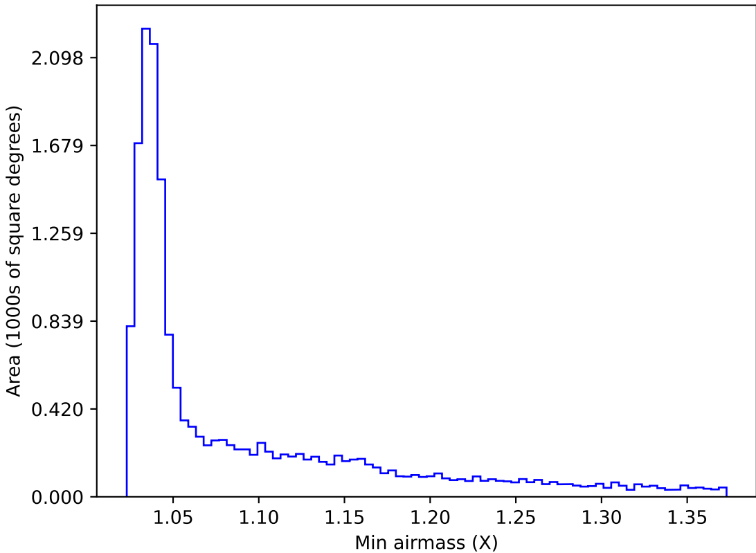
no_magell_roll_v3.4_10yrs WFD g band: Min airmass
