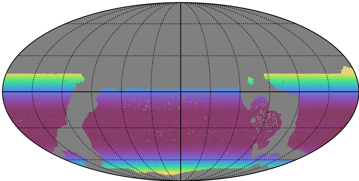
no_magell_roll_v3.4_10yrs WFD all bands: Min airmass
