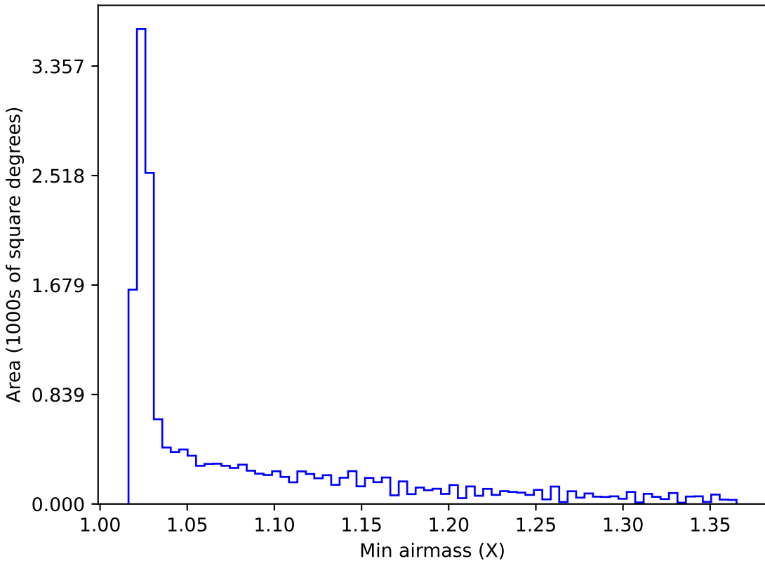
no_magell_roll_v3.4_10yrs WFD all bands: Min airmass
