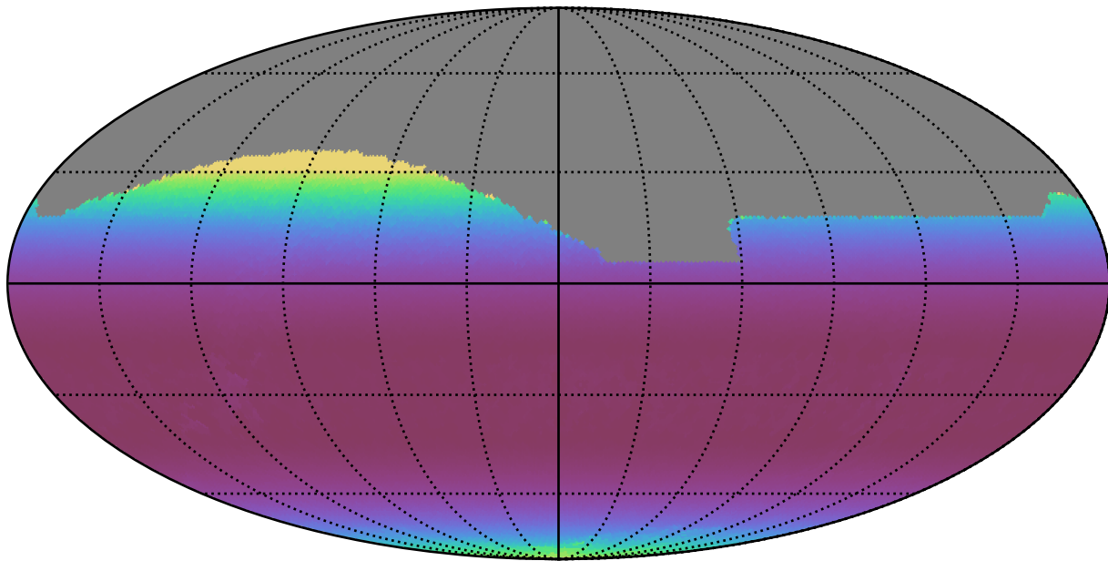
no_magell_roll_v3.4_10yrs All sky z band: Min airmass
